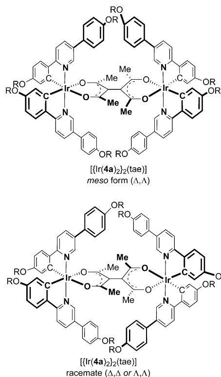
Figure 4. Structure of enantiomeric forms for complexes 5 with 5a as exemplar.
