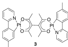
Figure 2. Example of a Pt(II)tae complex.
